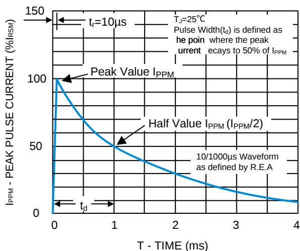
FIG.3 PULSE WAVEFORM
